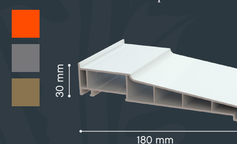
R007 180mm Cill R311 180mm Cill End Cap
