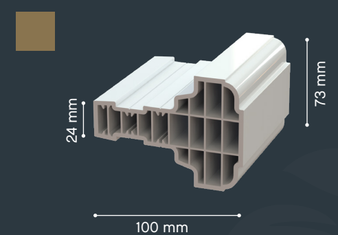
R001 Decorative Transom/Mullion
