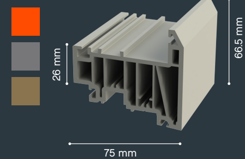
R003 Flush Window Sash
