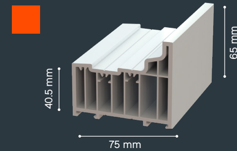
R7002 Residence 7 Frame
