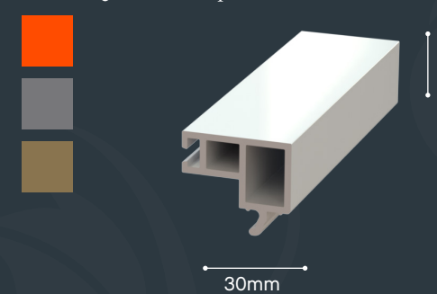
R004SQ 28mm Square Bead
