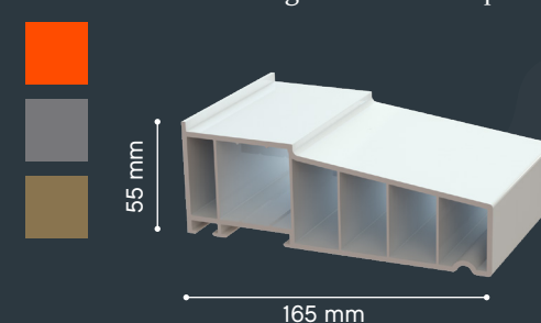
R009 55mm Radlington Cill R324 55mm Radlington Cill End Cap
