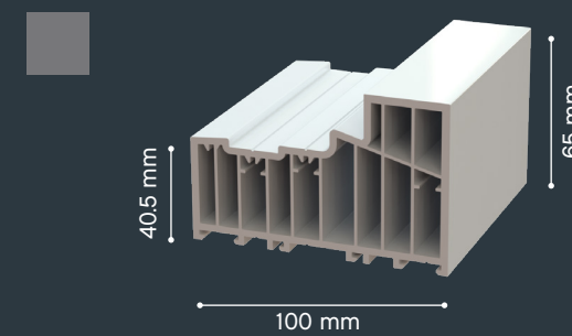
RS002 Residence 2 Frame
