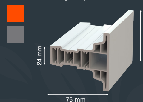
R001M Contemporary Transom/Mullion
