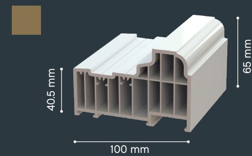
R002 Residence 9 Frame
