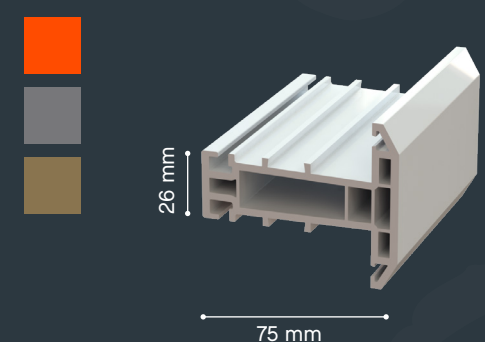
R001SM Sash Transom/Mullion
