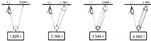
1.2) LIFTING – machine anchored to load
