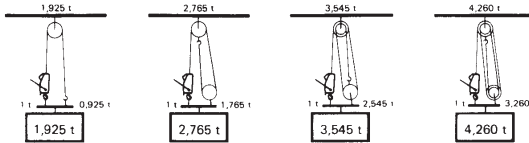
1.3) LIFTING – machine anchored at ground level
