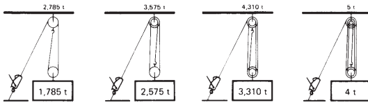
1.3) LIFTING – machine anchored at ground level
